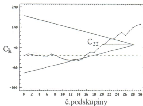
b) Diagram CUSUM
